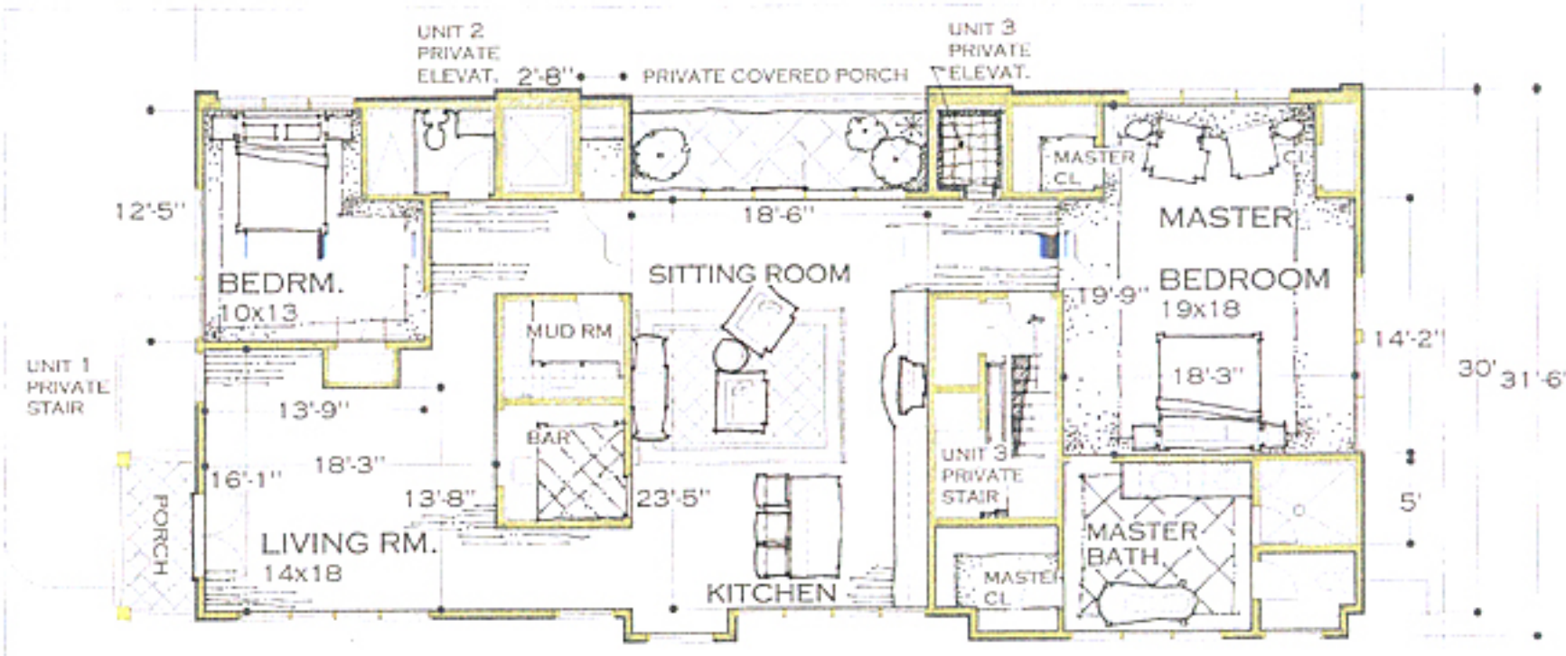
third level plan
