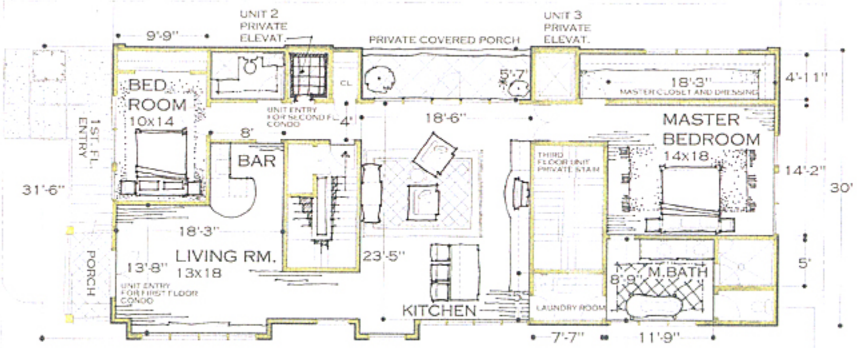
1st/ 2nd level plan
